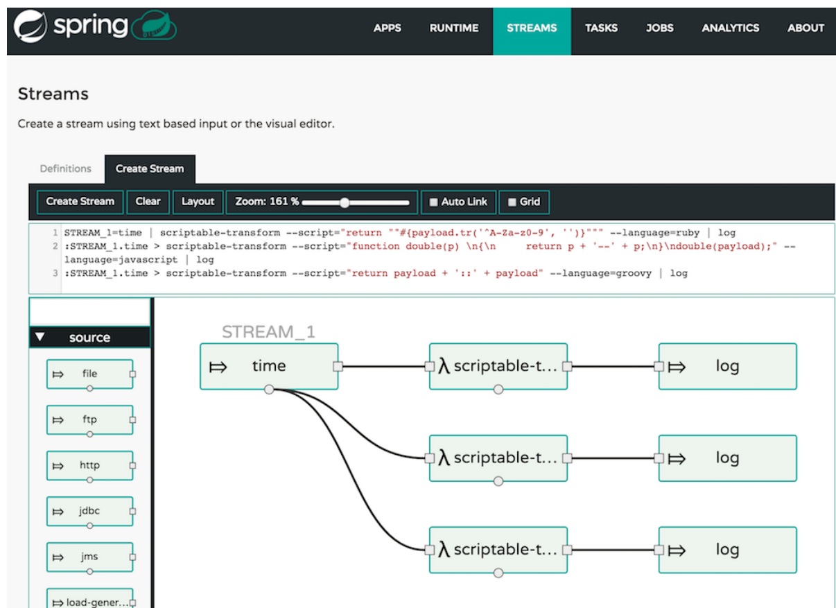
Figure 42.1. Flo for Spring Cloud Data Flow
