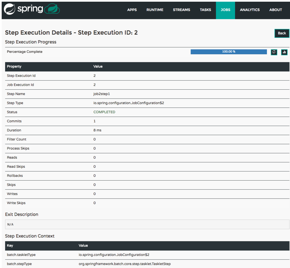
Figure 44.3. Step Execution History
