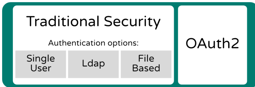
Figure 17.1. Authentication Options
