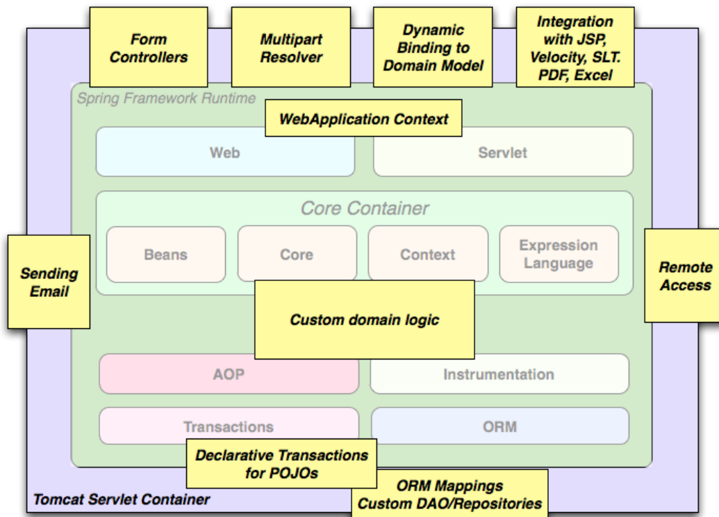
Typical full-fledged Spring web application
