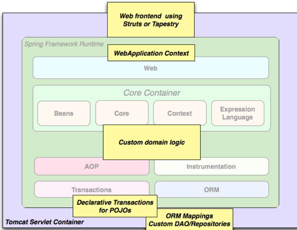
Spring middle-tier using a third-party web framework
