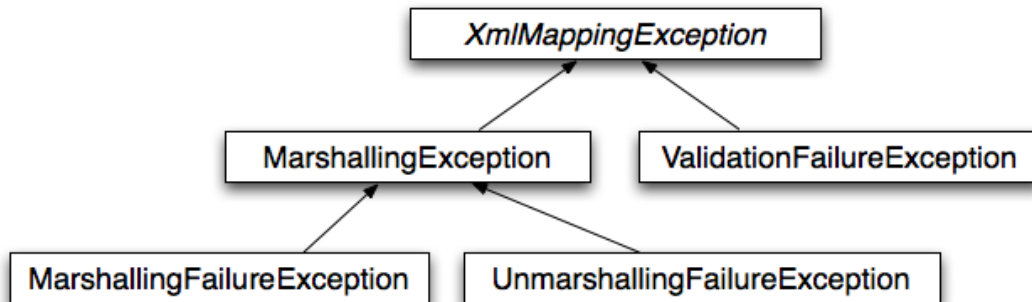
O/X Mapping exception hierarchy
