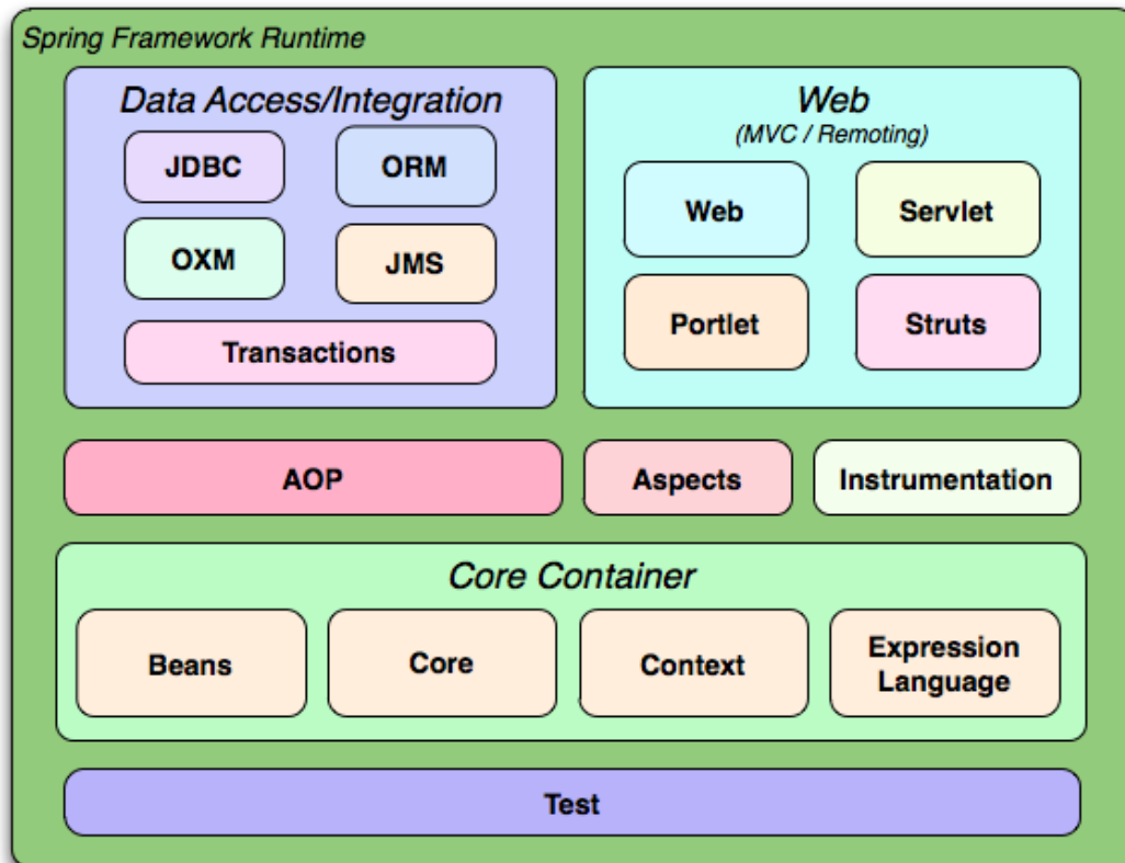
Overview of the Spring Framework
