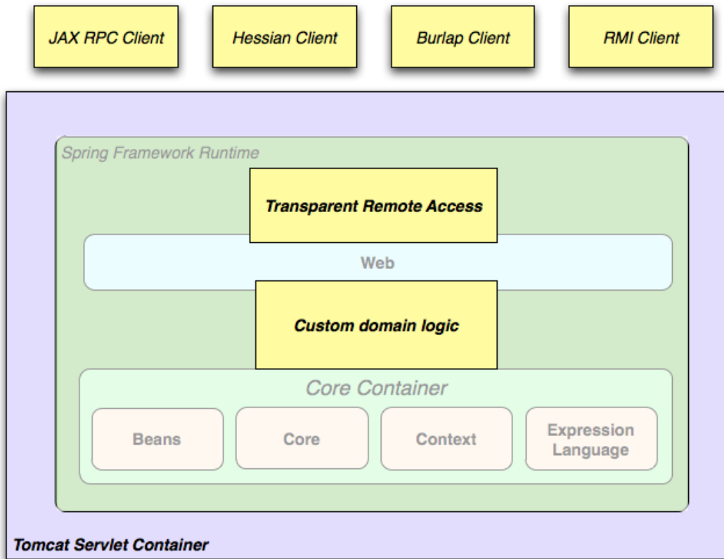
Remoting usage scenario
