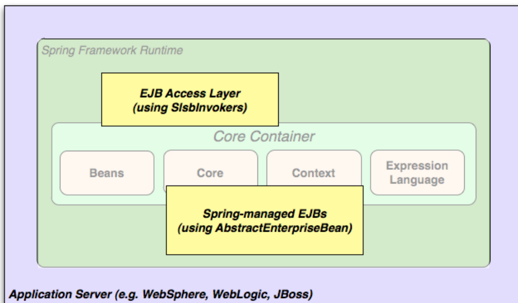
EJBs - Wrapping existing POJOs
