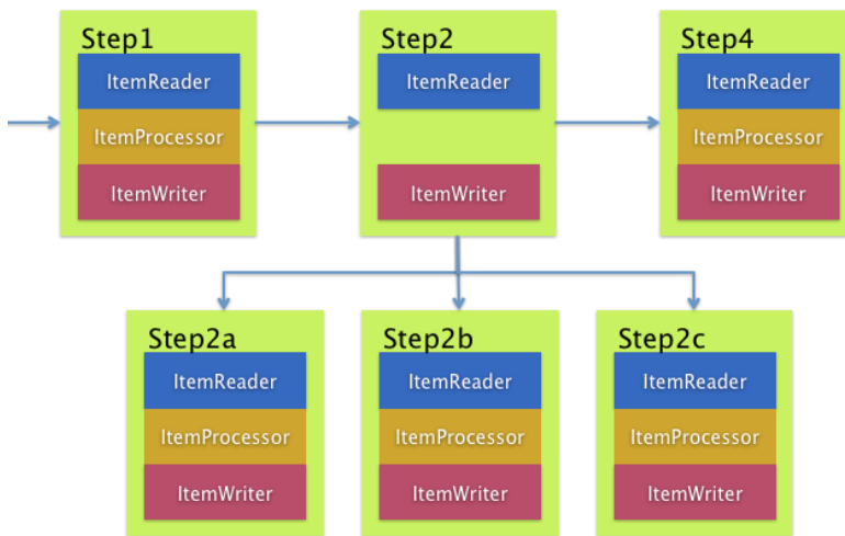
Figure 29. Remote Chunking
