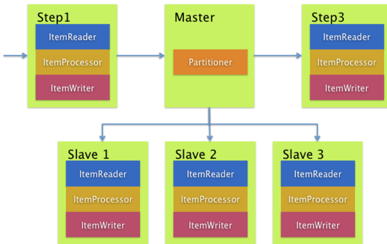
Figure 30. Remote Partitioning
