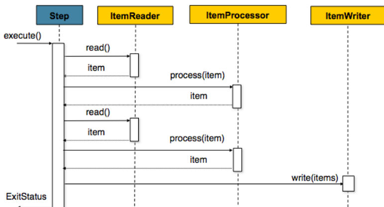
Figure 14. Chunk-oriented Processing
