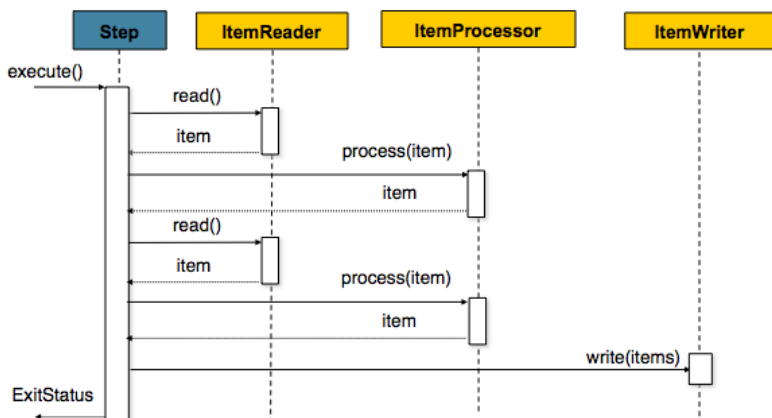
Figure 14. Chunk-oriented Processing
