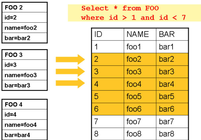
Figure 19. Cursor Example
