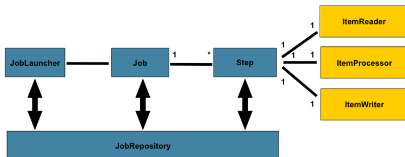
Figure 3. Batch Stereotypes
