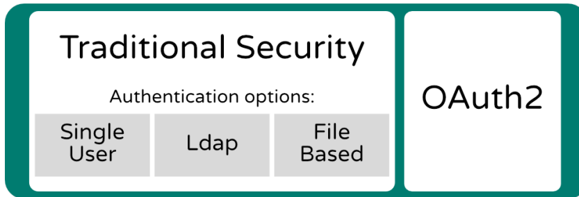
Figure 23.1. Authentication Options
