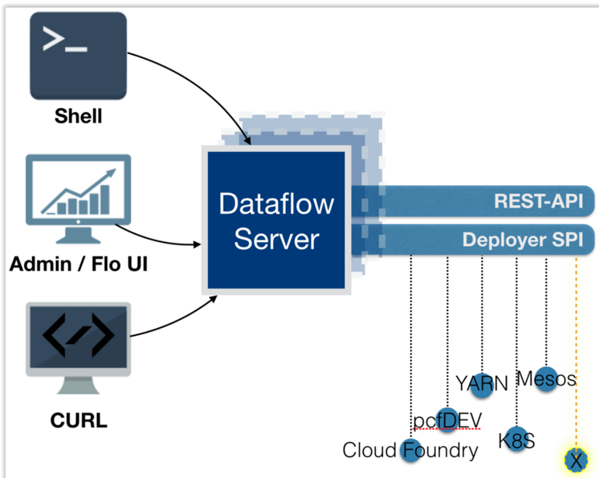
Figure 13.1. The Spring Cloud Data Flow Server
