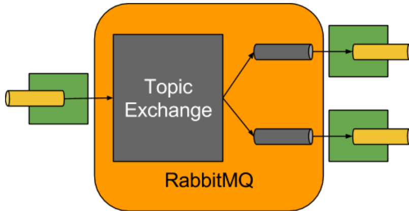
Figure 4.3. RabbitMQ Binder
