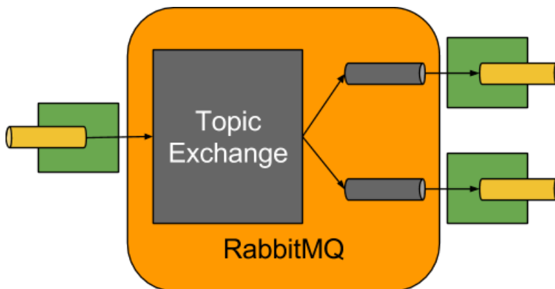
Figure 14.1. RabbitMQ Binder
