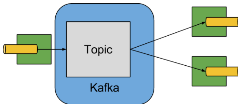
Figure 13.1. Kafka Binder
