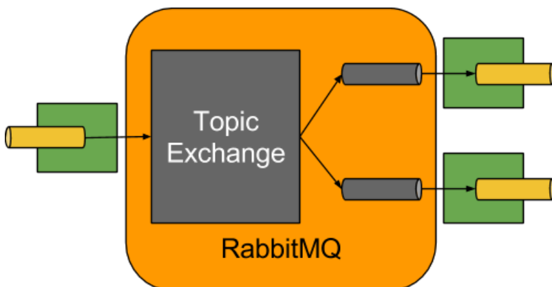
Figure 15.1. RabbitMQ Binder
