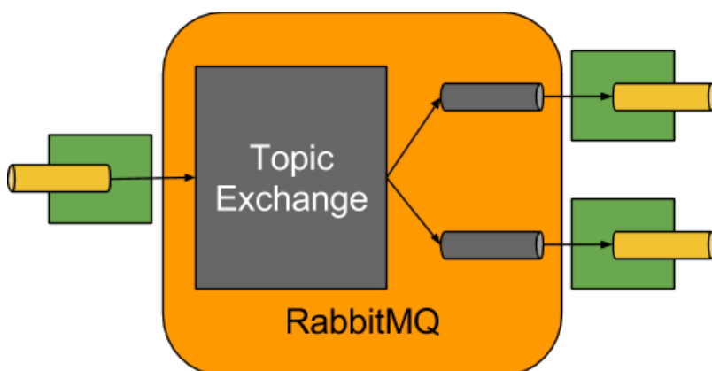
Figure 15.1. RabbitMQ Binder
