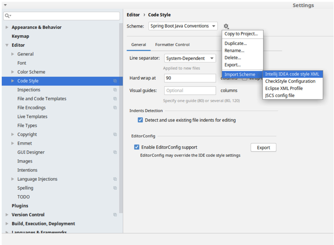
Figure 1. Code style
