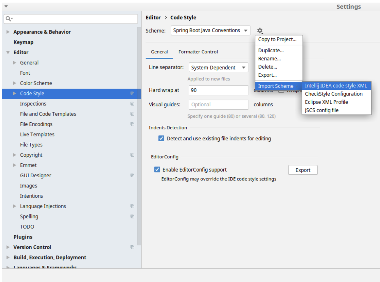
Figure 3. Code style
