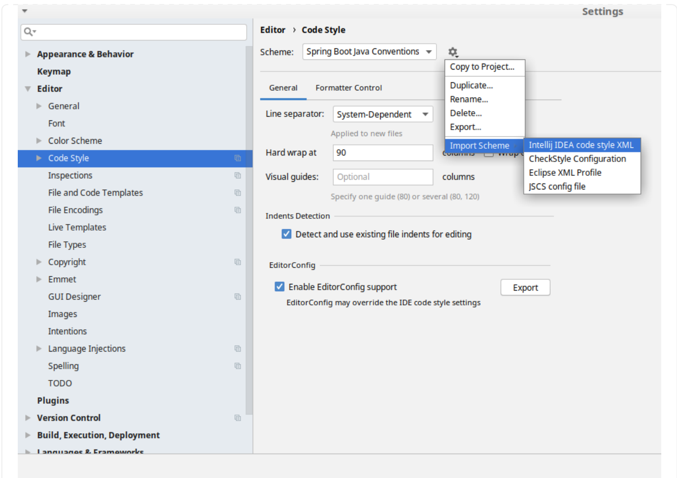
Figure 5. Code style
