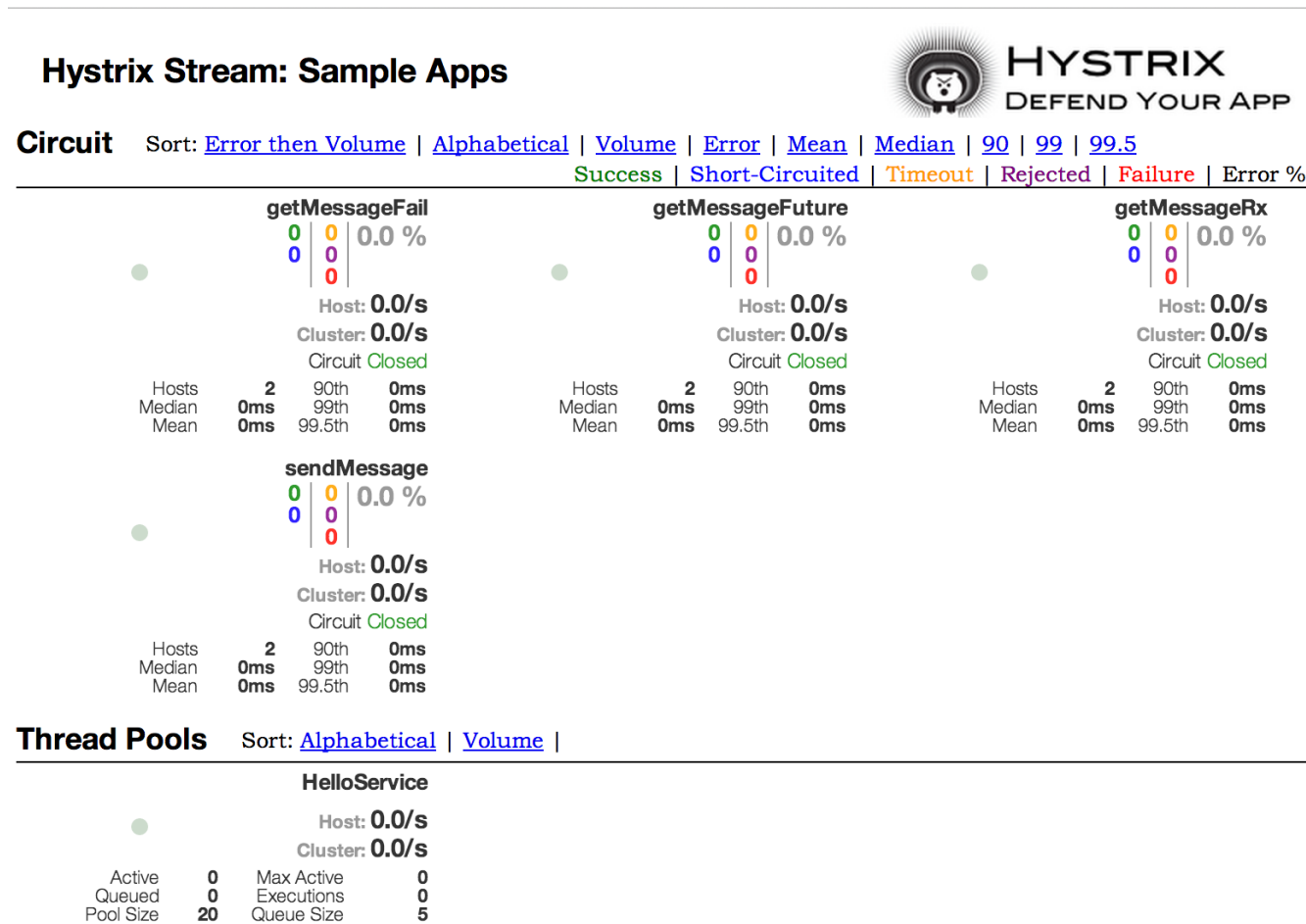
Figure 9. Hystrix Dashboard
