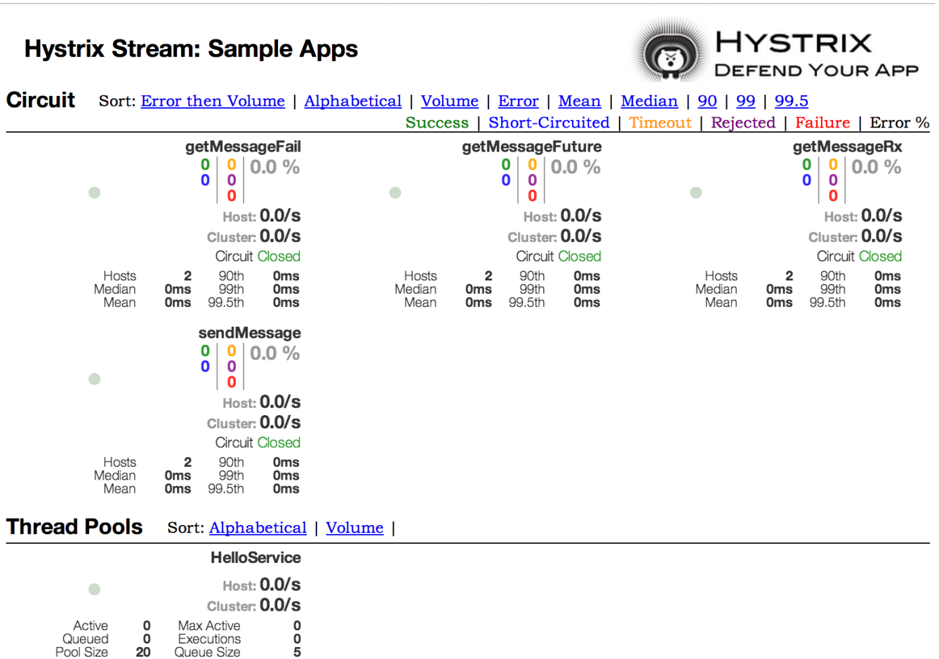
Figure 7. Microservice Graph
