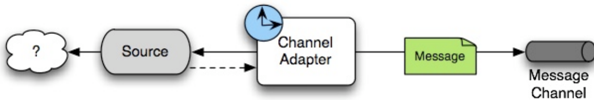
Figure 3.4. An inbound "Channel Adapter" endpoint connects a source system to a MessageChannel.
