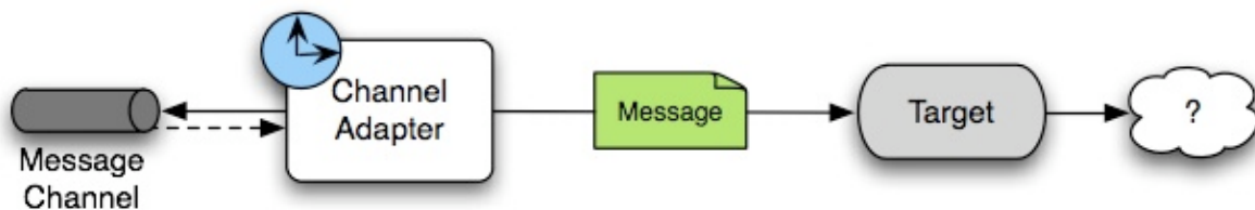
Figure 3.5. An outbound "Channel Adapter" endpoint connects a MessageChannel to a target system.
