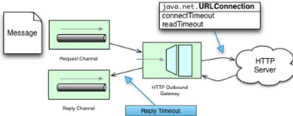
Figure 17.2. How timeout settings apply to an HTTP Outbound Gateway
