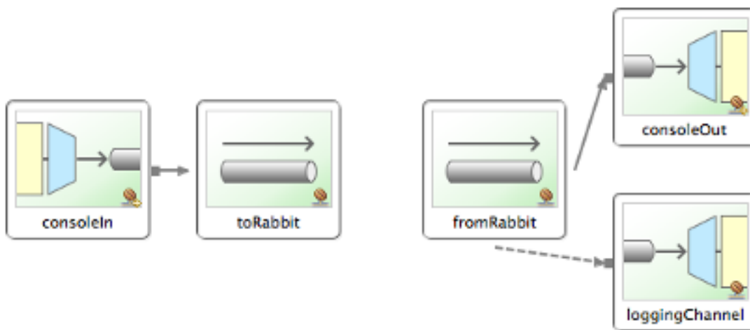
Figure 11.1. The Spring Integration graph of the AMQP sample
