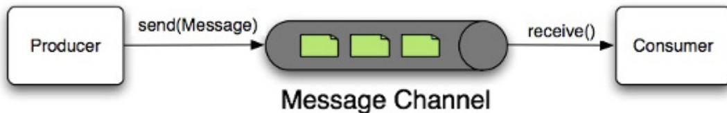
Figure 2. Message Channel
