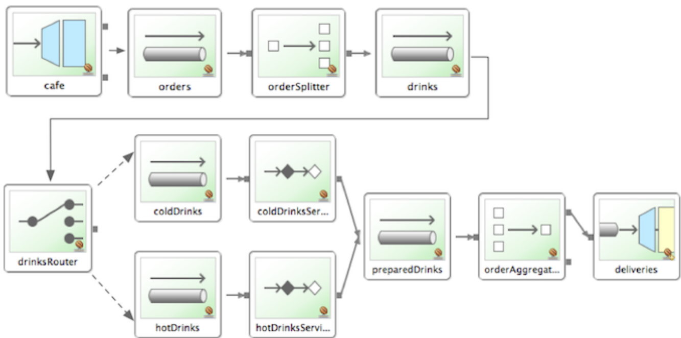
Figure 15. Cafe Sample
