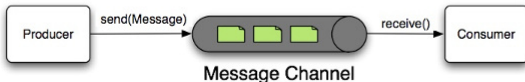
Figure 2. Message Channel
