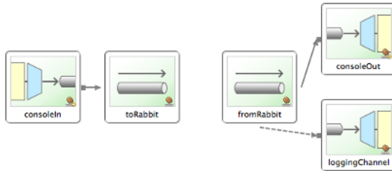
Figure 7. The Spring Integration graph of the AMQP sample
