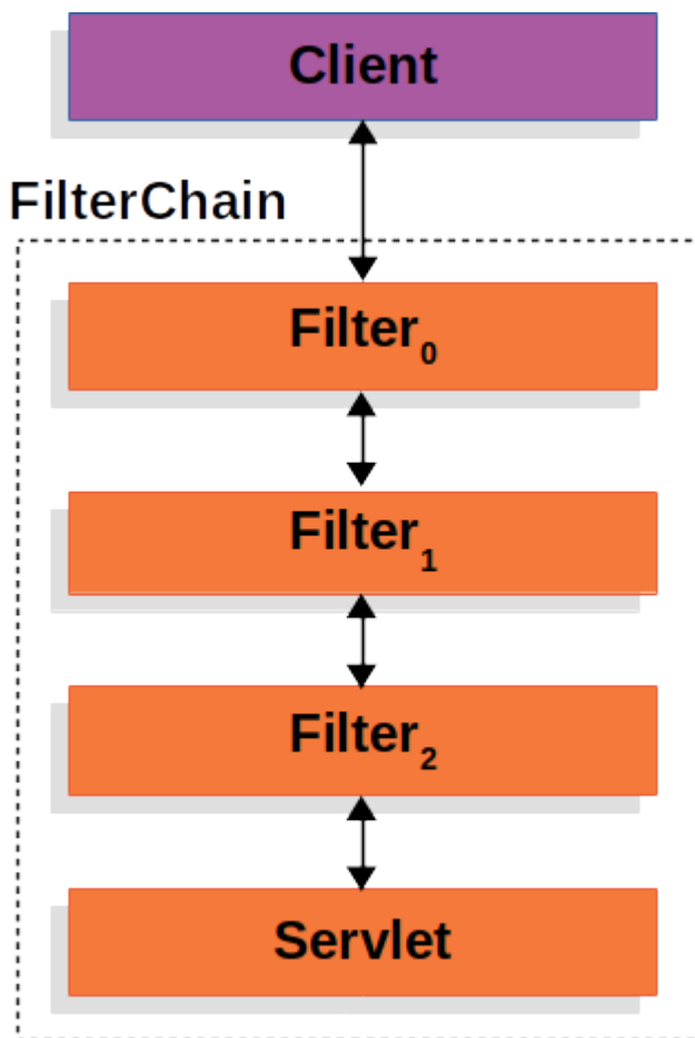
Figure 1. FilterChain
