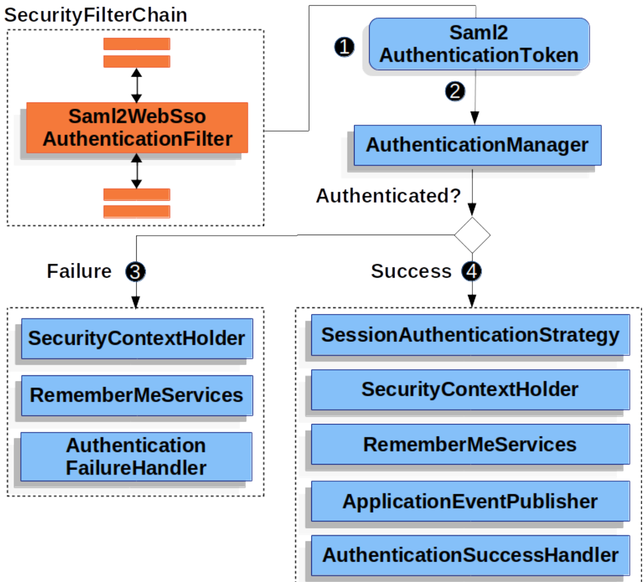
Figure 19. Authenticating a <saml2:Response>
