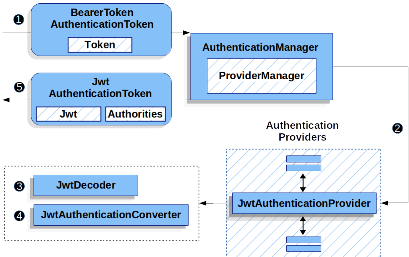
Figure 16. JwtAuthenticationProvider Usage
