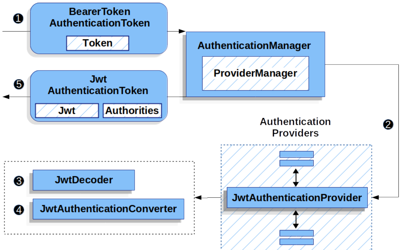
Figure 16. JwtAuthenticationProvider Usage
