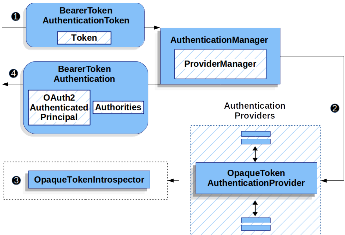
Figure 17. OpaqueTokenAuthenticationProvider Usage
