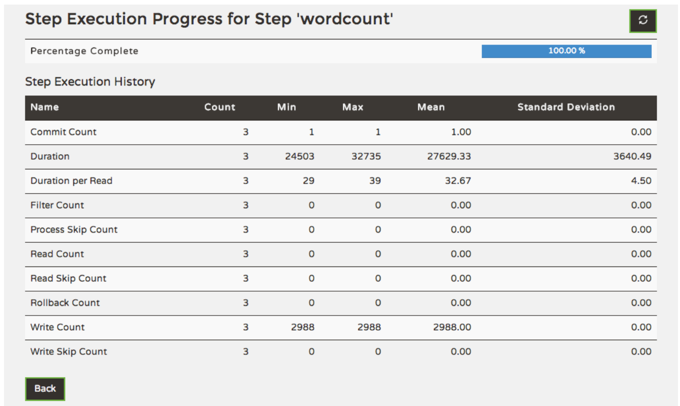
Figure 21.17. Step Execution History
