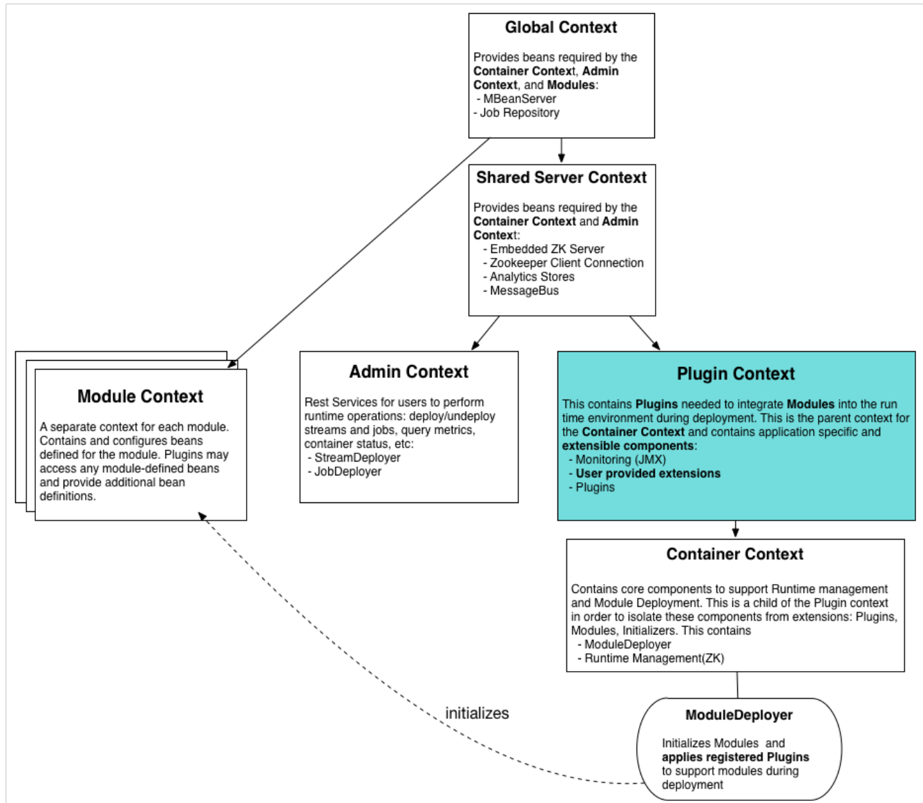
Figure 25.1. The Spring XD Application Context Hierarchy
