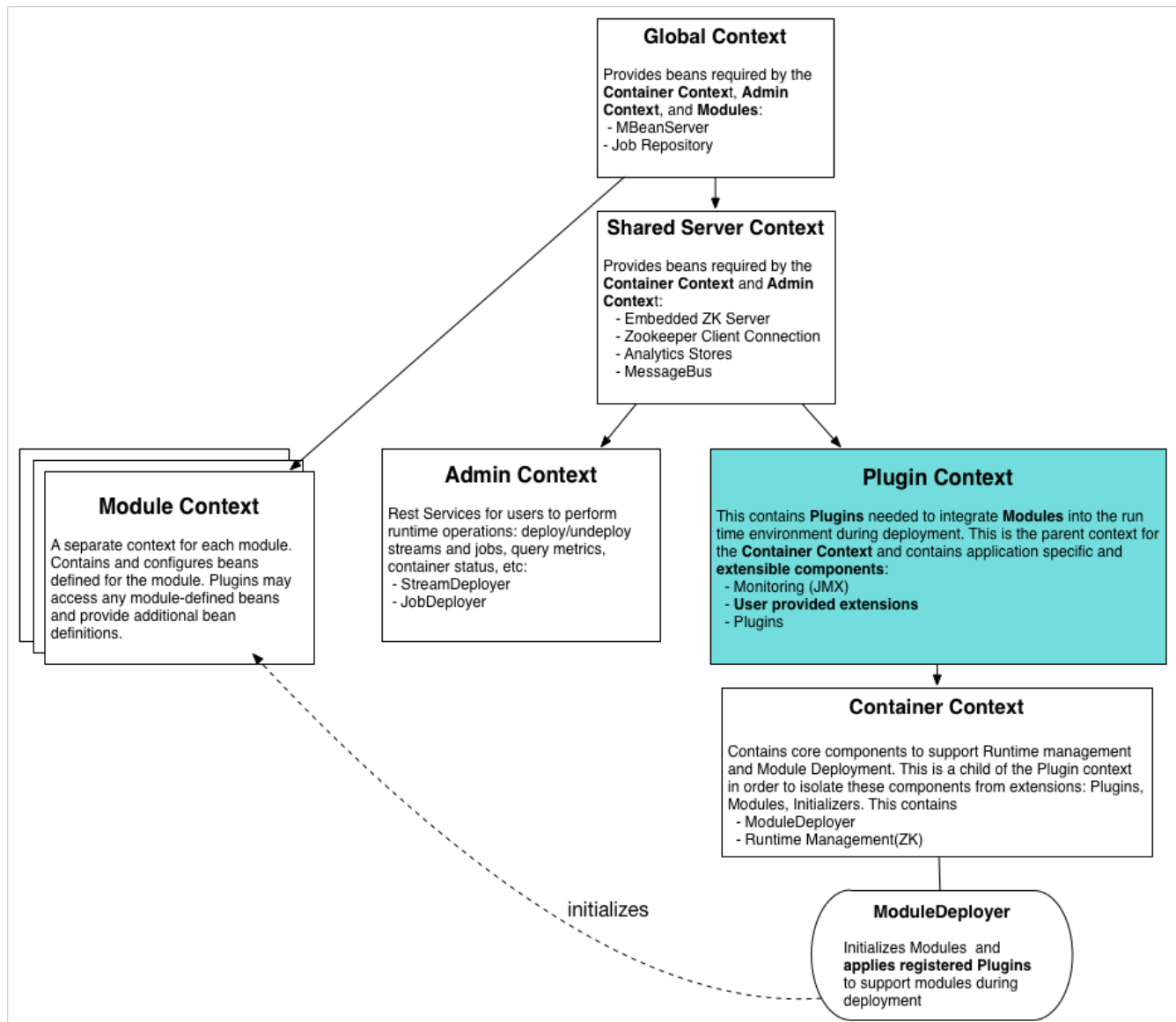
Figure 31.1. The Spring XD Application Context Hierarchy
